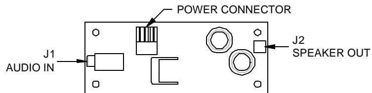
Figure 32 - Audio Amp Board Drawing
