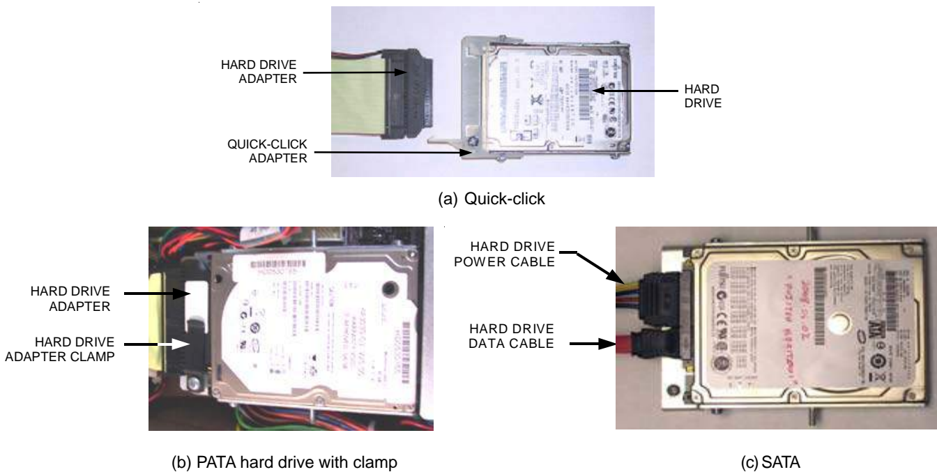
FIGURE 1 - HARD DRIVES
