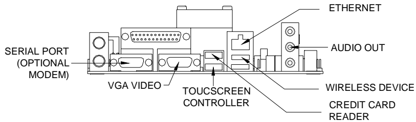
CONNECTOR SIDE VIEW OF MOTHERBOARD
