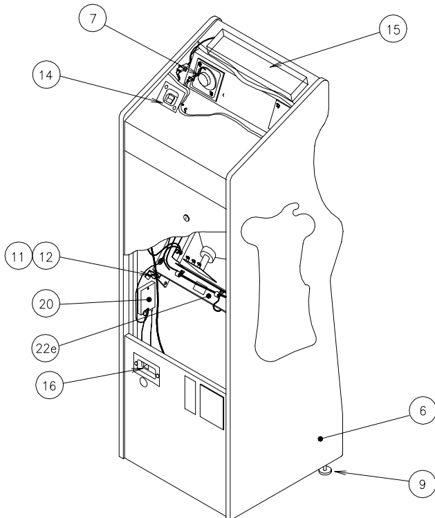
FIGURE 14 - 19" CABARET (REAR VIEW)
